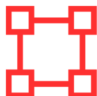
USABILITY TESTING
