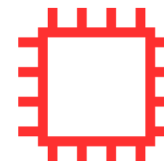
CONFIGURATION TESTING
