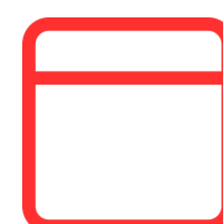
BLACK-BOX TESTING
