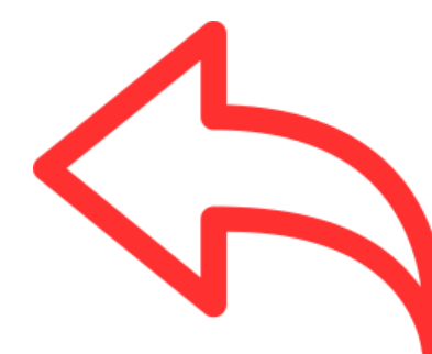
REGRESSION TESTING
